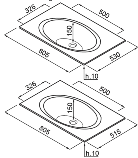
Technical Drawing
